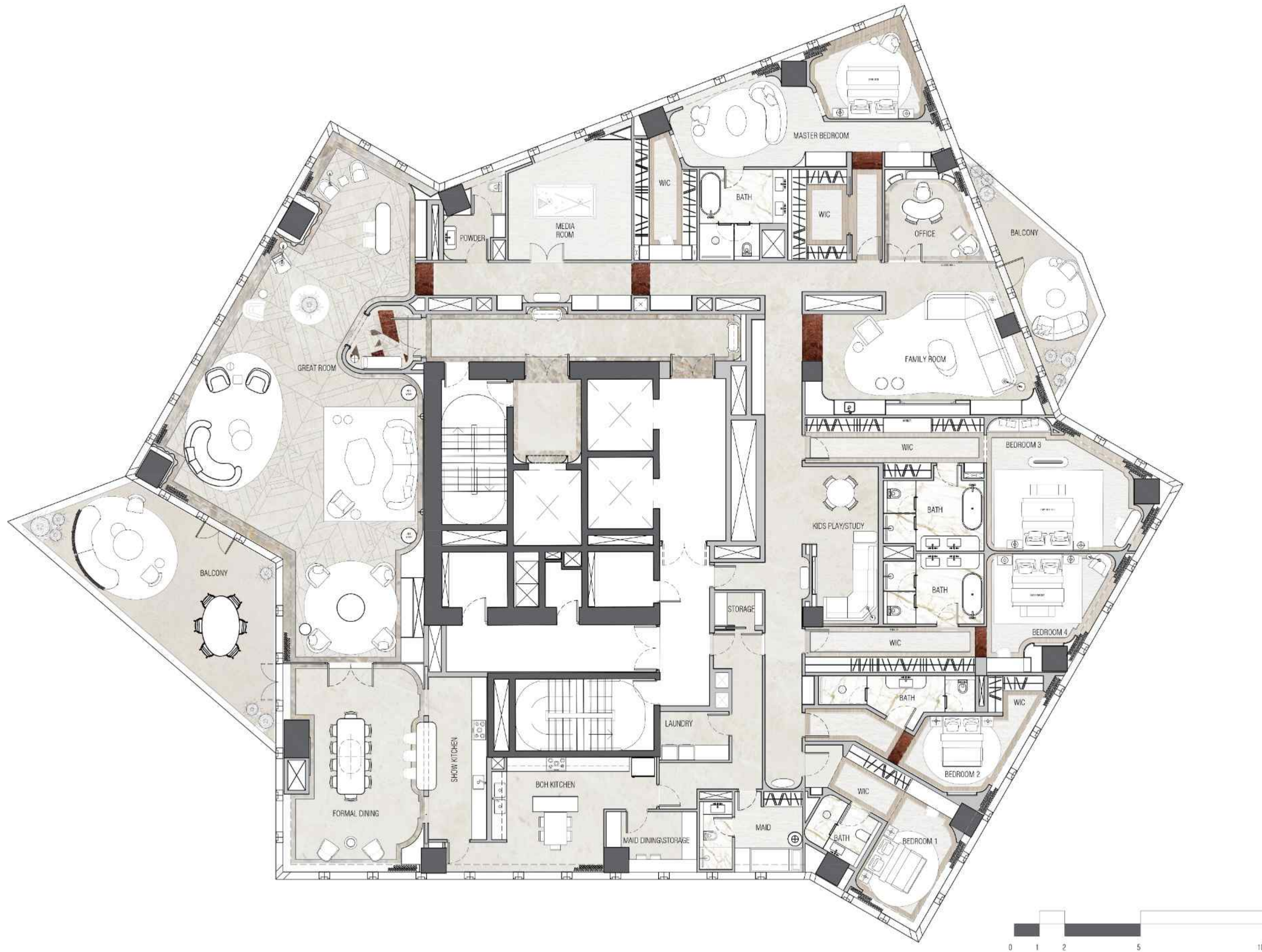
1 FL-39 PENTHOUSE APARTMENT GENERAL ARRANGEMENT PLAN 1:100
